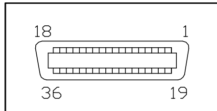
Centronics Parallel
